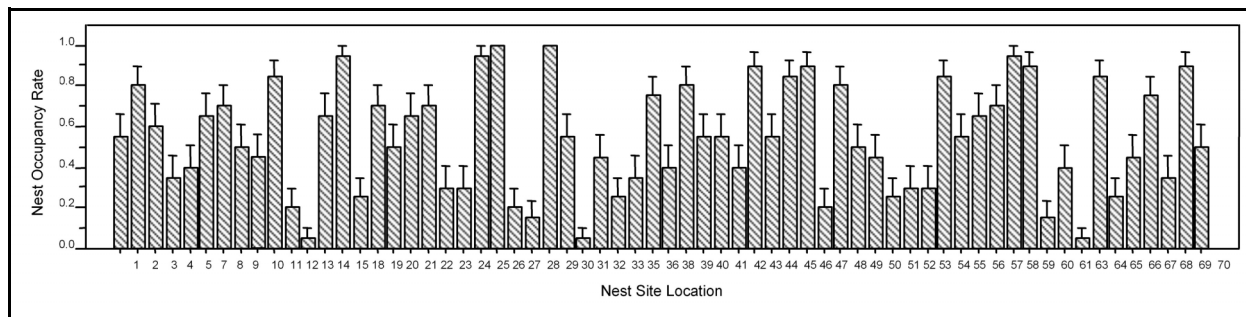
Figure 4. Nest occupancy rate for 64 Xantus's murrelet nests, Cat Canyon, Santa Barbara, 1983 – 2002.
