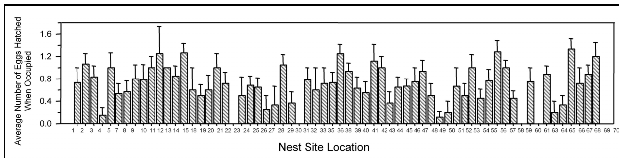
Figure 5. Average number of eggs hatched when a nest was occupied for 64 Xantus's murrelet nests, 1983–2002, Cat Canyon, Santa Barbara Island.
